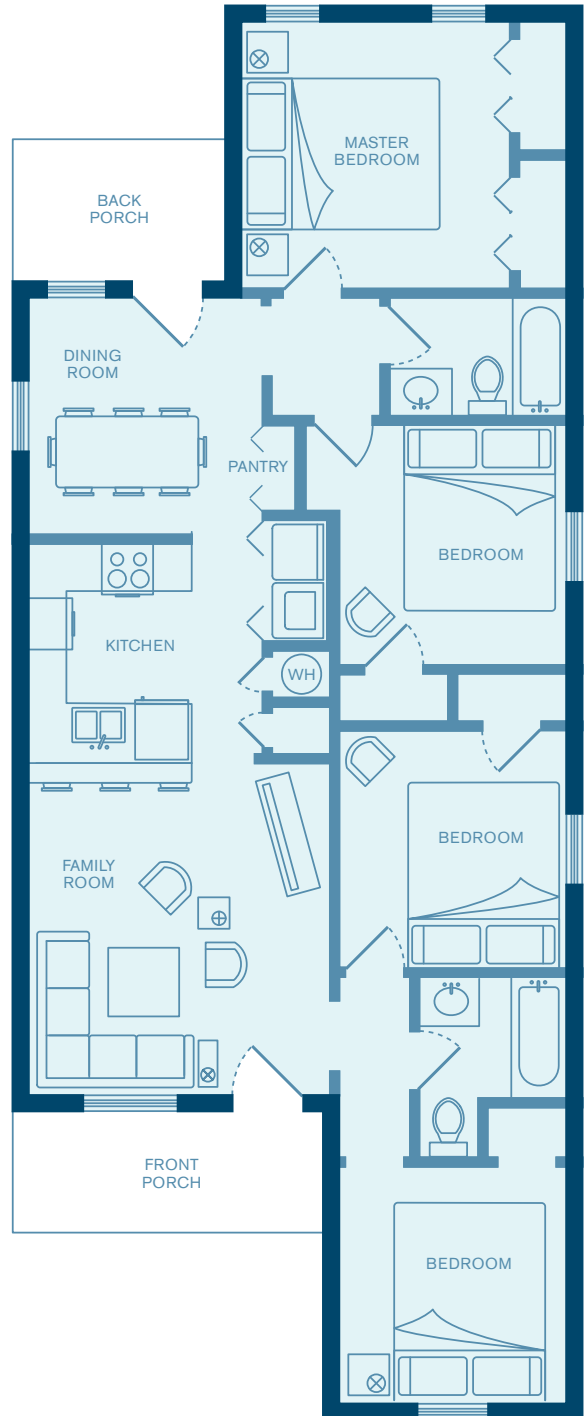
SAMPLE FLOOR PLAN
